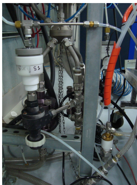
Filter pack (white, marked S1) with cyclone (black) below
