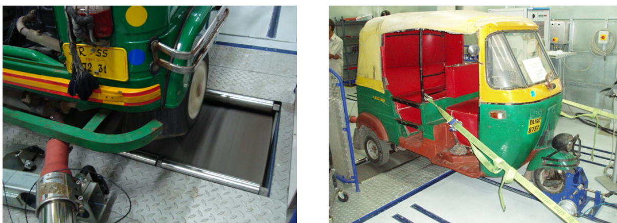
Figure 8: Autorickshaw on chassis dyno
