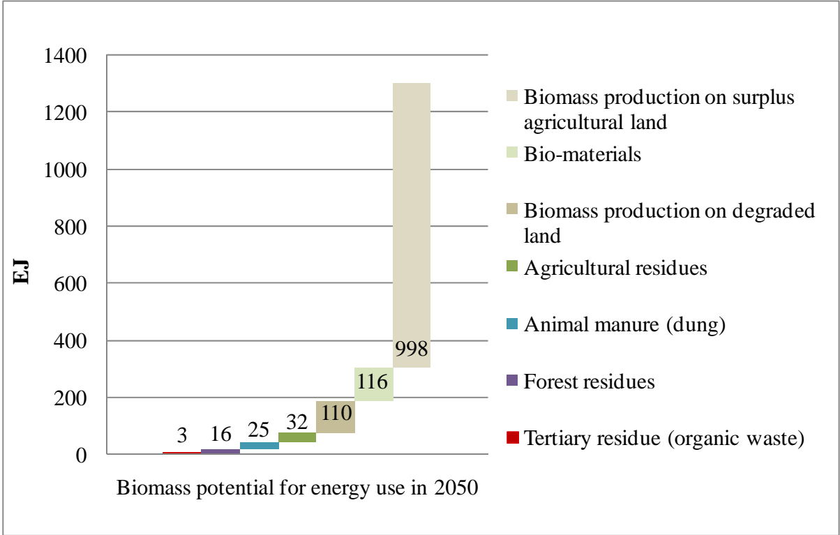
Figure 9. Contribution of each biomass resource category to the global potential of biomass for energy use in 2050 (Source: Hoogwijk et al, 2003).
