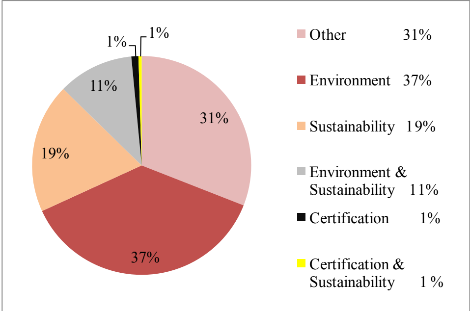
Figure 3. Relative distribution of records of different criteria within 4,911 renewable bioenergy records (Source: renewable energy Topic a in all databases of ISI Web of Knowledge refined by bioenergy Topic c as well as different criteria Topics e ).
