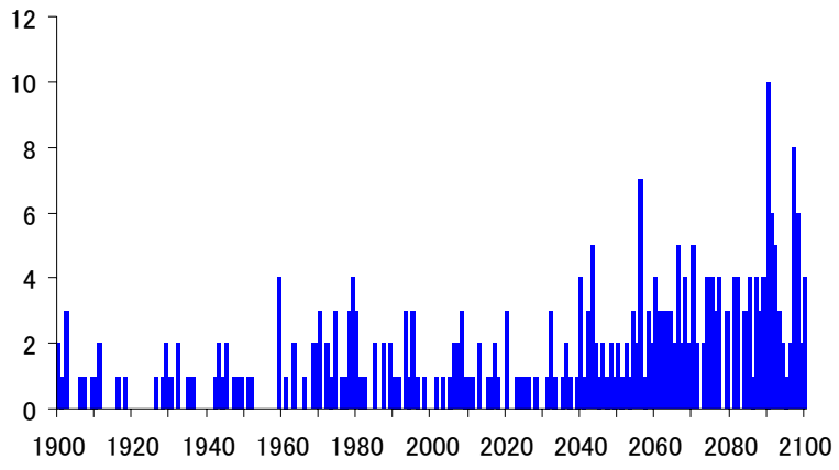
Figure 19 Number of summer days with extreme rainfalls in Japan (unit: days) (Combined research team(Tokyo University etc.),2004)
