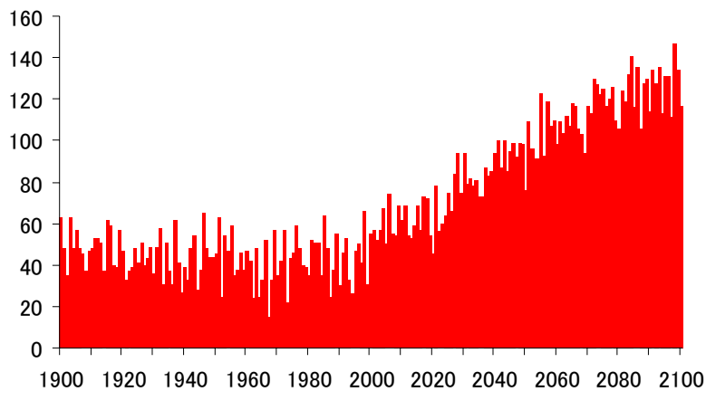
Figure 18 Number of hot days (maximum temperature is more than 30 C) in Japan (unit: days) (Combined research team(Tokyo University etc.),2004)
