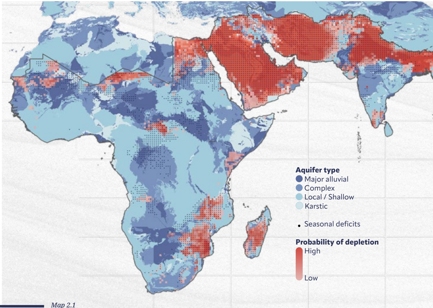
Map 2.1 Declining trends and seasonal groundwater deficits using downscaled GRACE satellite data
